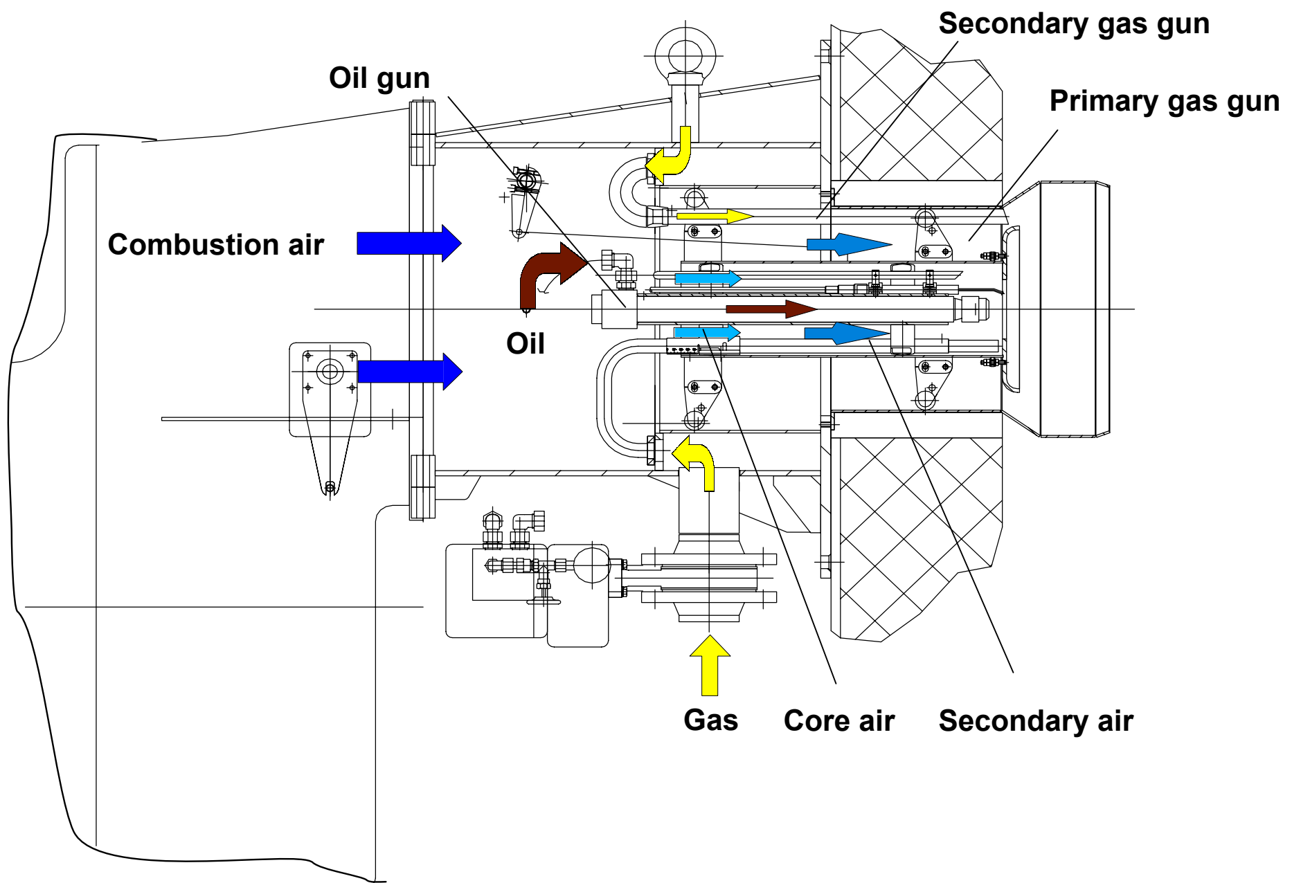
Combined low NO x burner (gas/LFO) for GWK/WRK TEMINOX ® -GLS
