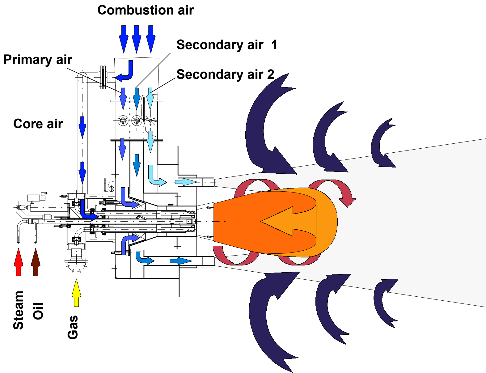
Combined low NO x burner (gas/oil) for WRK with steam-assisted pressure jet burner DDZG-TF
