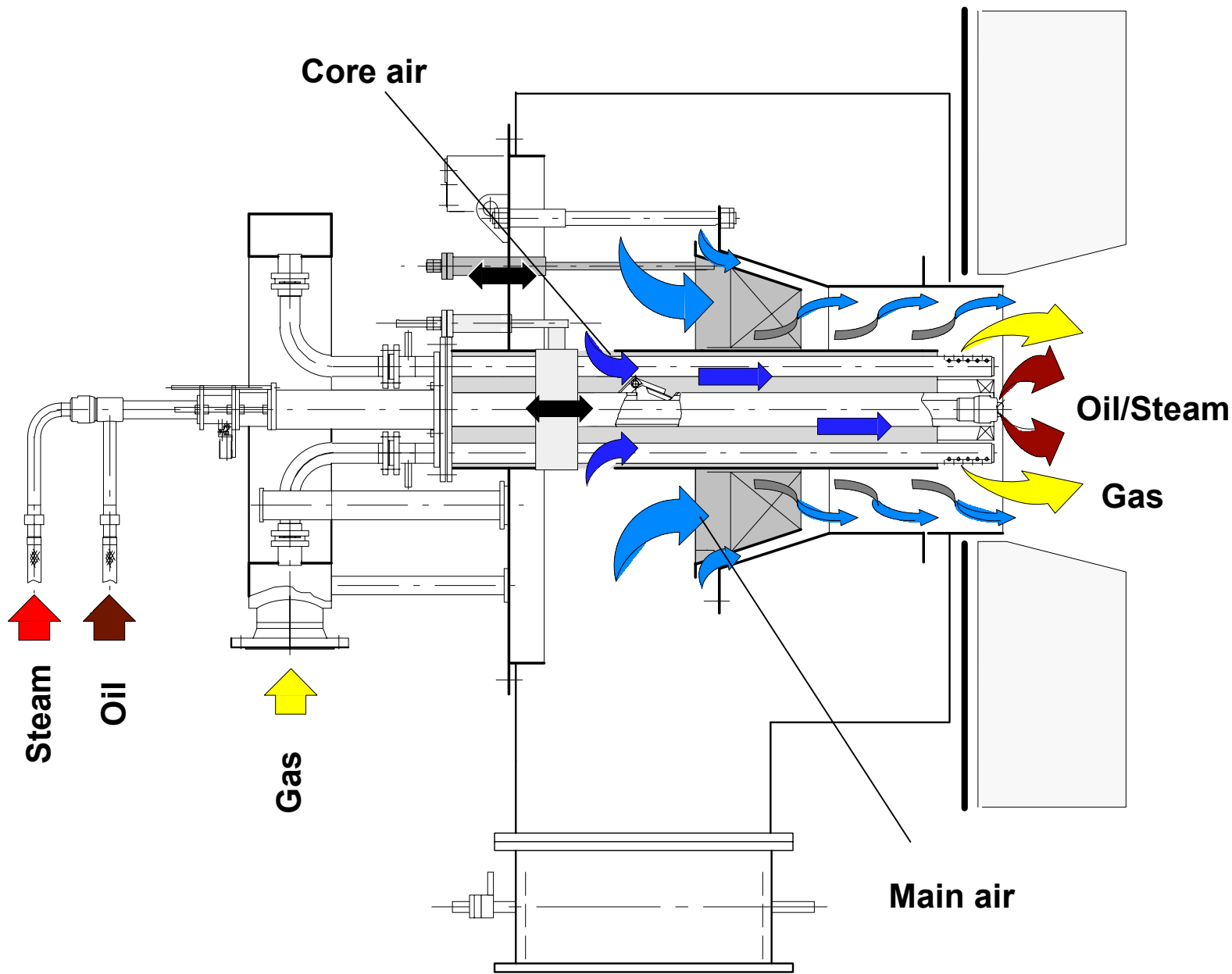
Duoblock combined with steam-assisted pressure jet burner DDZG
