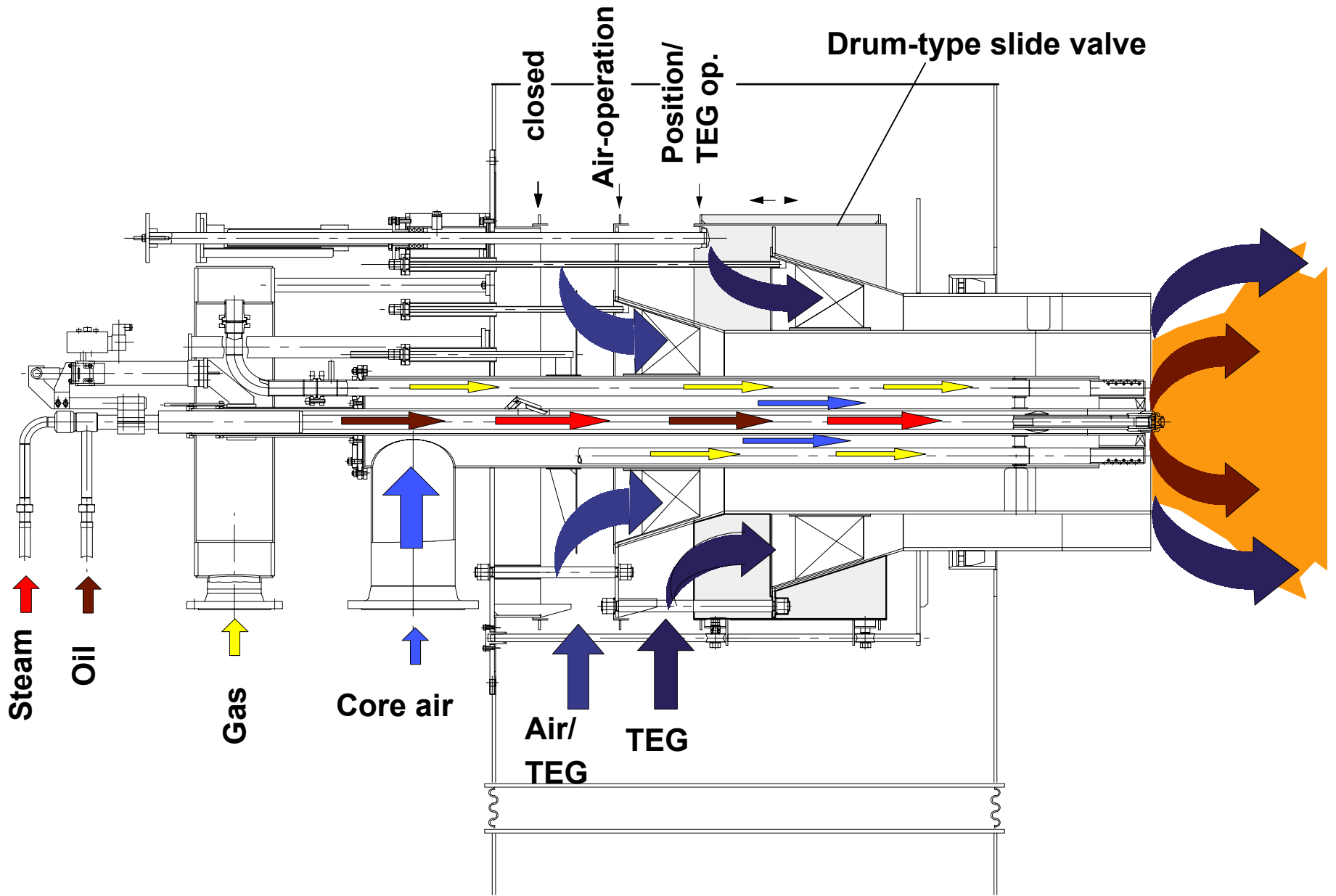
Additional firing system for gas turbine exhaust gas(TEG) DDZG-GT
